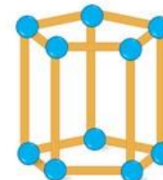
Prisma pentagonal
