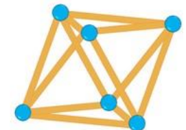
Octaedro
