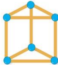
Prisma triangular
