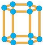
Prisma hexagonal
